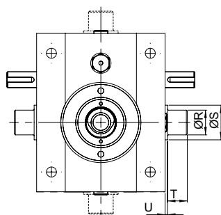
Female Trunnion
