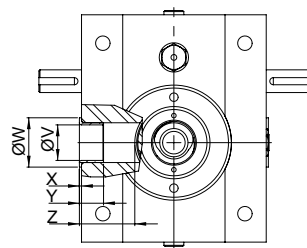
Male Trunnion
