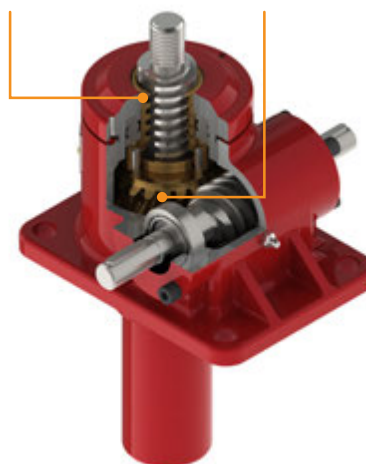
Anti-Backlash Nut
