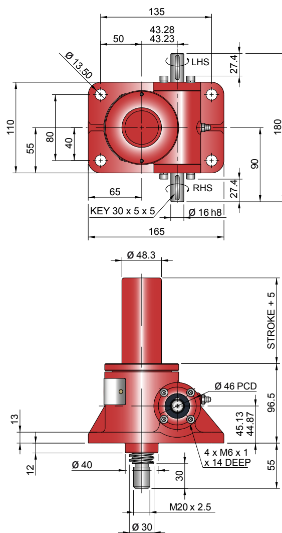
Inverted EMT0025-I00
