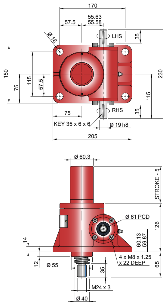
Inverted EMT0050-I00
