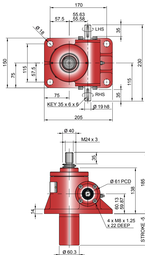
Upright EMT0050-U00
