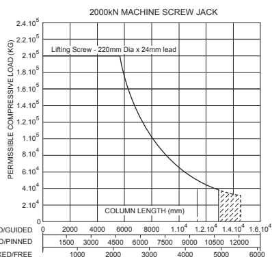
Column Strength
