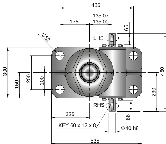
Upright EMT0500-V00
