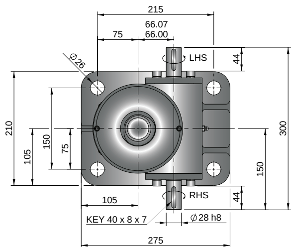
Upright EMT0200-V00
