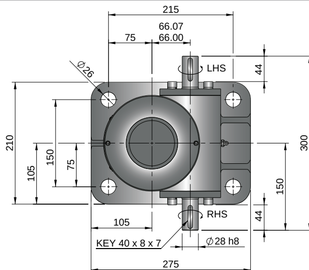
Inverted EMT0200-J00
