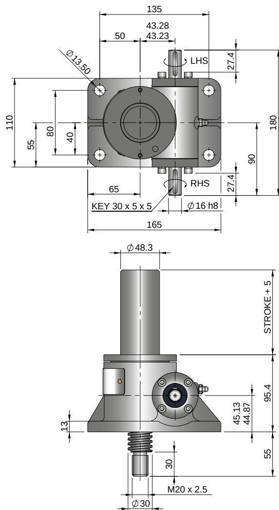
Inverted EMT0025-J00
