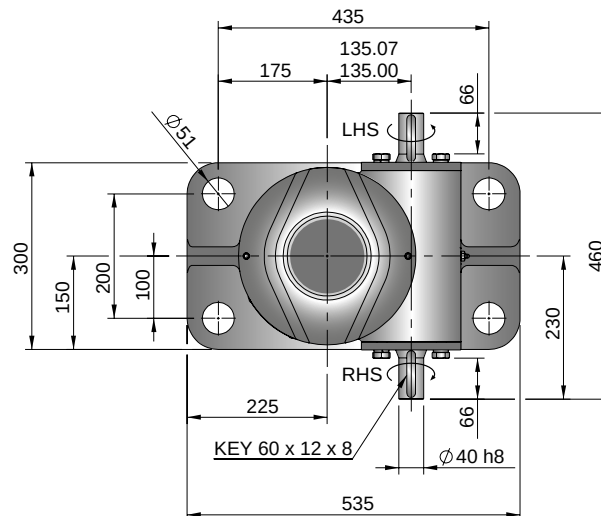
Inverted EMT0500-J00
